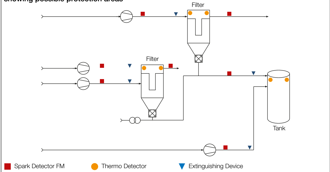
Diagram of a furniture production process showing possible protection areas
