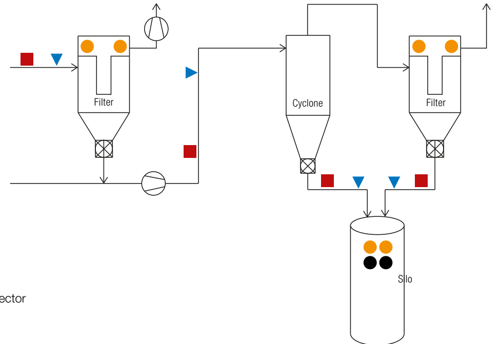
Diagram of a plywood production process showing possible protection areas
